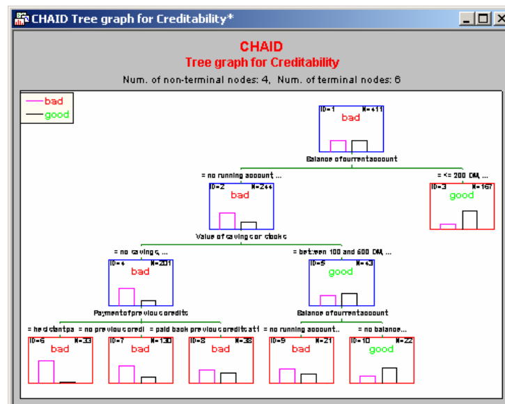
CHAID decision tree for “Creditability”
