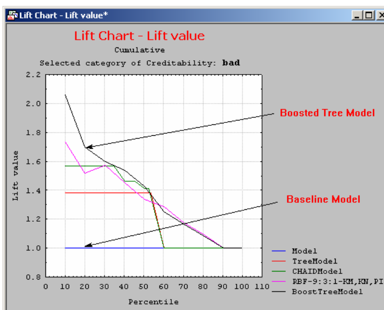
Lift Chart for “Creditability” = “Bad”
