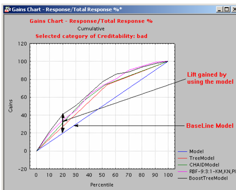
Gains Chart for “Creditability” = “Bad”
